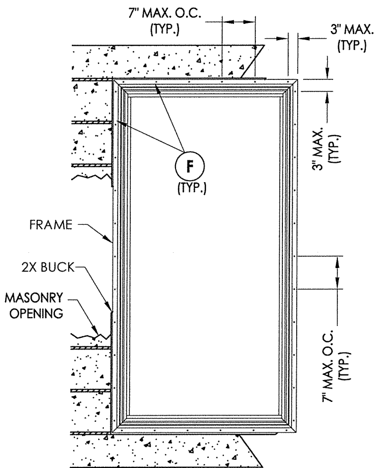
FRAME ANCHORING 2X Buck Masonry Construction
