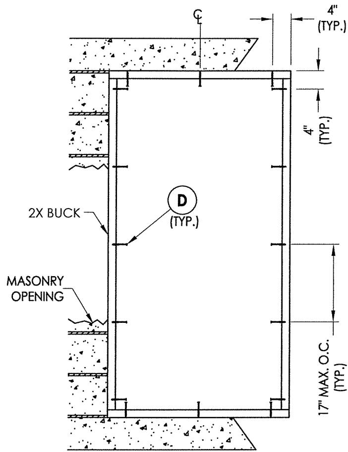
BUCK ANCHORING 36" x 72"
