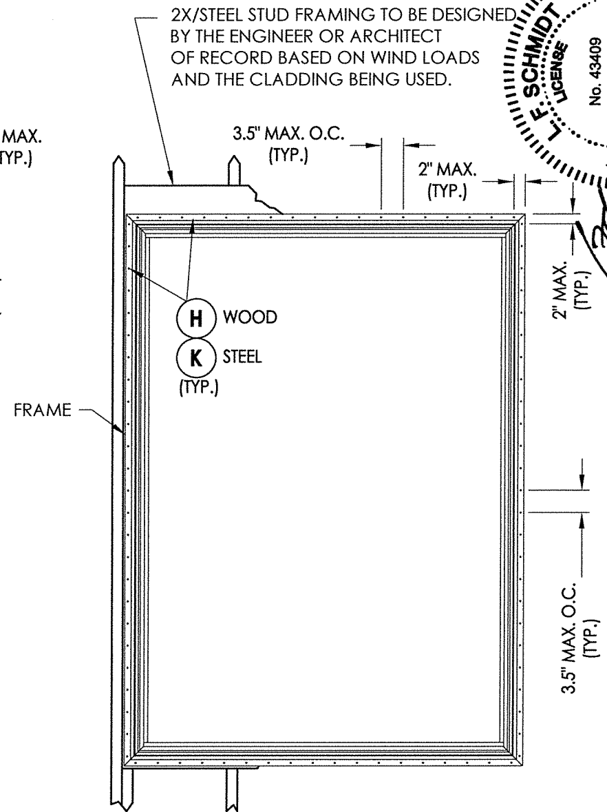
FRAME ANCHORING Stud Construction
