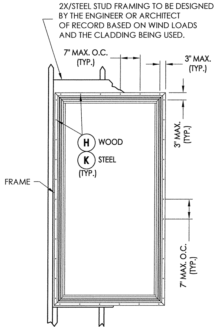
FRAME ANCHORING Stud Construction
